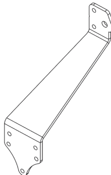
1x Plate Top Link, LH AA-1004
