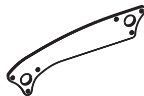
2x Plate, Toolbar Mount AA-1202
