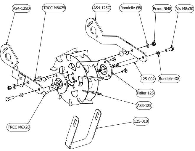
T.CG.RS120s Taille/Size 120mm
