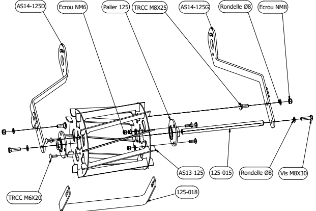
T.CG.RS270s Taille/Size 270mm
