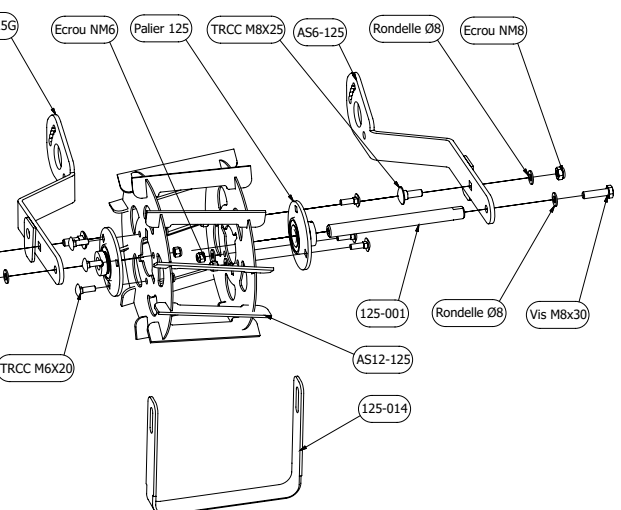
T.CG.RS180s Taille/Size 180mm
